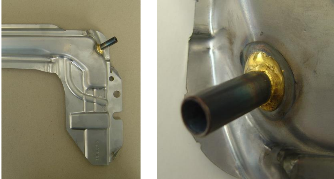
Fig. 1 Left – view of roof window car component, right – the close-up of MIG CMT brazed joint
